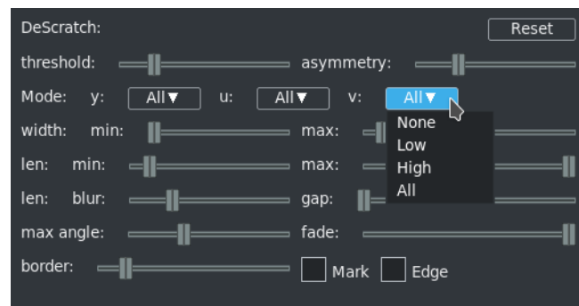
Figure 10.37: DeScratch control window
