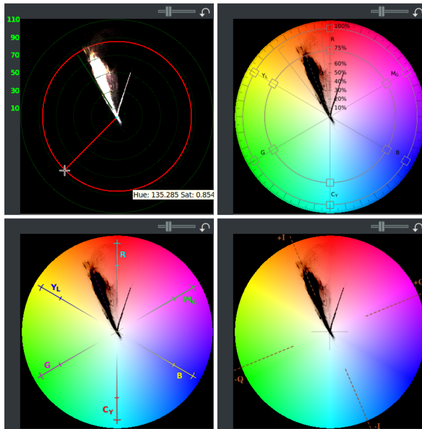
Figure 10.76: Vectorscope (with H/S pop-up box) and VectorWheel (with 3 default grids)
