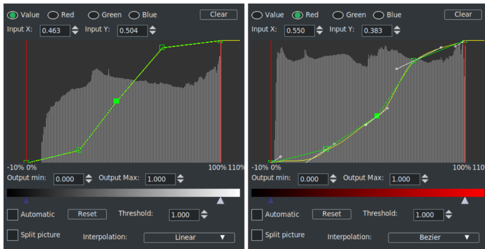
Figure 10.47: Histogram Bezier / Curves
