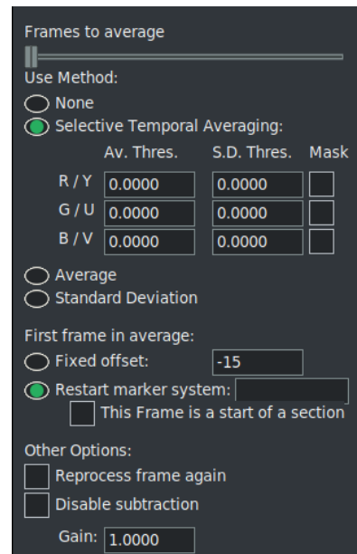
Figure 10.61: STA control window
