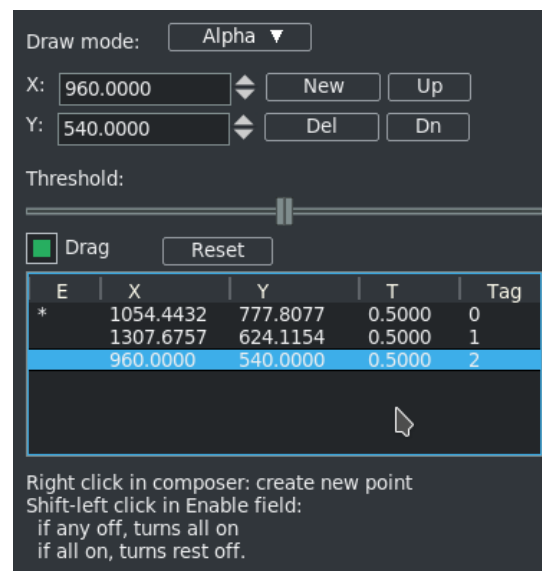
Figure 10.33: three active point created in CriKey
