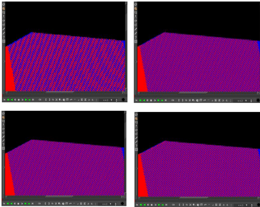
Figure 10.55: Clockwise: Nearest; Linear; OpenGL and Cubic
