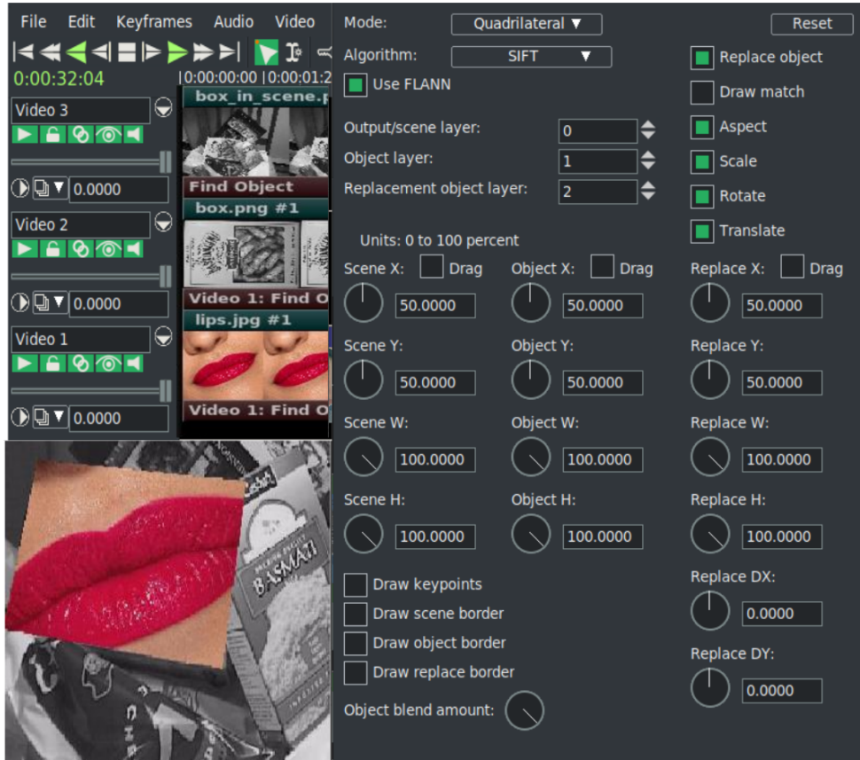
Figure 10.82: Timeline; control window and compositor for FindObj
