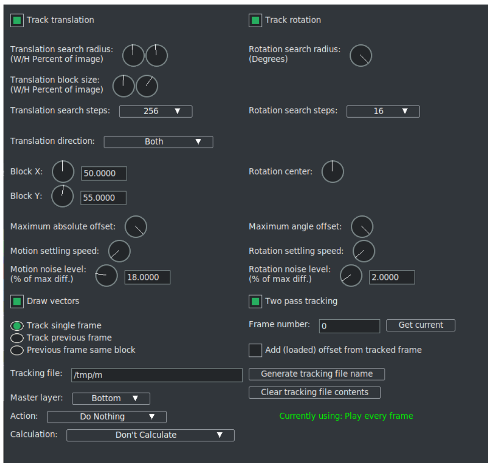
Figure 10.53: Motion plugin GUI
