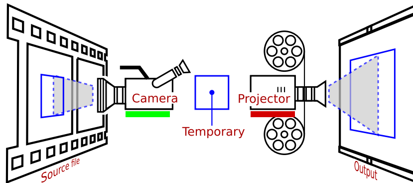
Figure 2.12: Compositing pipeline
