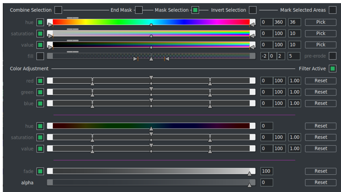
Figure 10.26: Screenshot showing the BlueBanana plugin control
